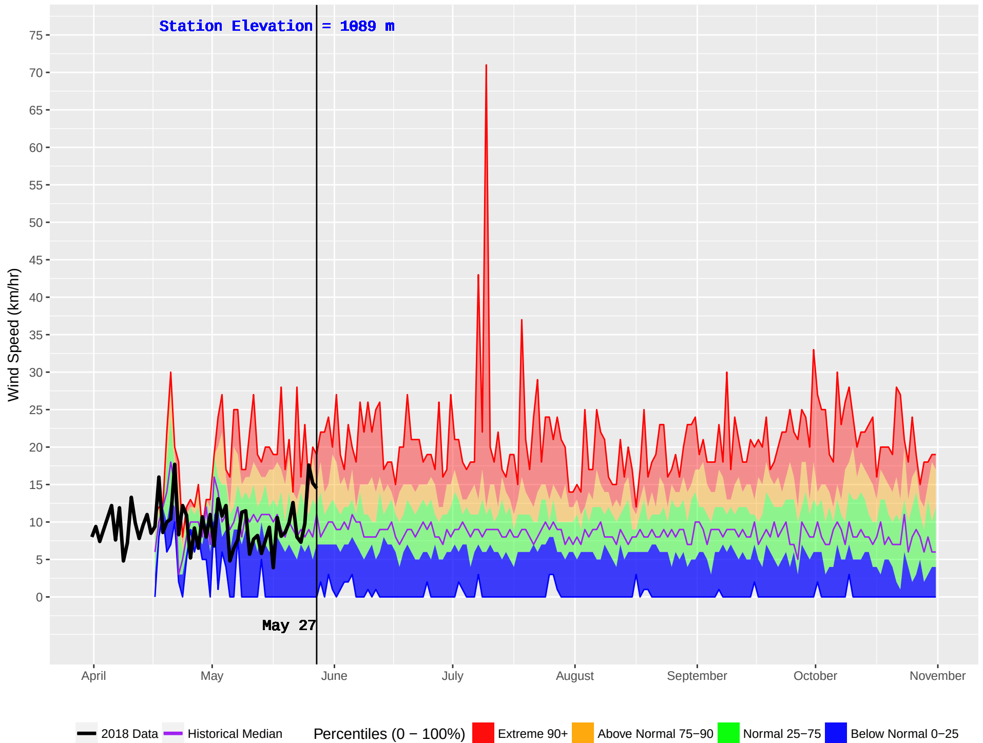
EAST OOTSA (170) : Historical (1986–2016) and Current (2018) Noon Wind Speed
